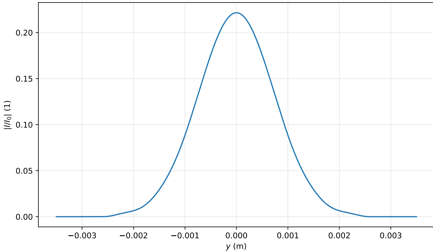
Intensity profile I(x=0, y, z=3.981)/I_0 , P_{in}=0.1P_{cr} , artificial time
